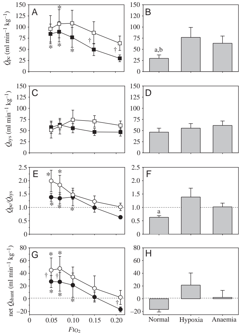
Fig. 3. Effects of hypoxia ( F_{\text{I}O_2} =fraction of oxygen in the inspired air) on blood flows before and after reducing haematocrit (filled and unfilled circles, respectively). (A,B) Pulmocutaneous blood flow ( \dot{Q}_{\text{pc}} ); (C,D) systemic blood flow ( \dot{Q}_{\text{sys}} ); (E,F) net shunt fraction ( \dot{Q}_{\text{pc}}/\dot{Q}_{\text{sys}} ) and (G,H) net shunt flow ( \dot{Q}_{\text{shunt}} ). The dotted lines represent the condition where there is no net shunt. Significant effects of hypoxia within each of the two groups (normal and low haematocrit, respectively) are marked with an asterisk, and significant differences between the groups are marked with a dagger. B, D, F and H show data for toads with normal [\text{O}_2] during normoxia, toads with normal [\text{O}_2] during hypoxia ( F_{\text{I}O_2}=0.10 ), and anaemic toads during normoxia. Significant differences between normoxic and hypoxic animals are marked with 'a', and differences between normoxic and anaemic animals are marked with 'b'. Data are presented as means \pm 1 S.E.M. ( N=6 ).
