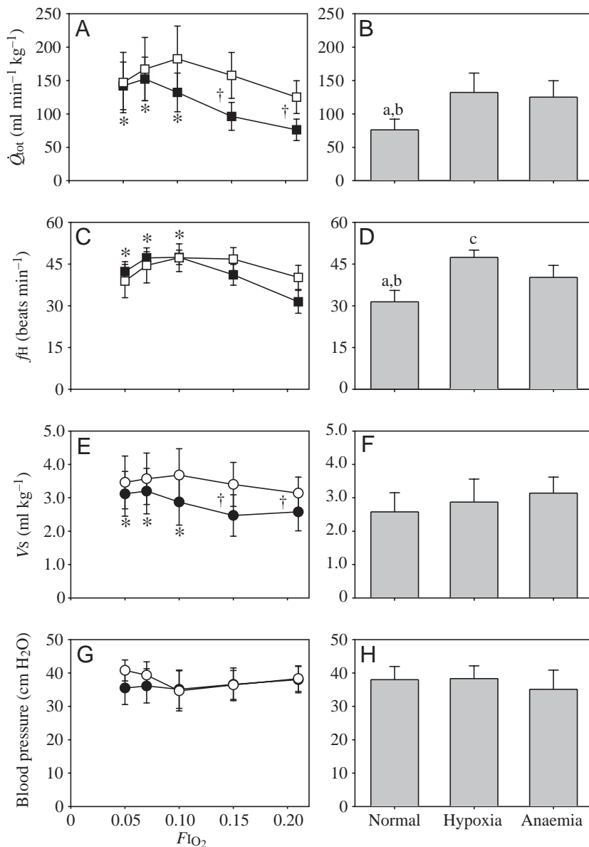
Fig. 4. Effects of hypoxia ( F_{\text{IO}_2} =fraction of oxygen in the inspired air) on heart parameters before and after a 50% reduction in haematocrit (filled and unfilled circles, respectively). (A,B) Total cardiac output ( \dot{Q}_{\text{tot}} ); (C,D) heart rate ( f_{\text{H}} ); (E,F) stroke volume ( V_{\text{s}} ) and (G,H) systemic blood pressure (1 cm H 2 O=98.1 Pa). Significant effects of hypoxia within each of the two groups (normal and low haematocrit, respectively) are marked with an asterisk, and significant differences between the groups are marked with a dagger. B, D, F and H show data for toads with normal [\text{O}_2] during normoxia, toads with normal [\text{O}_2] during hypoxia ( F_{\text{IO}_2}=0.10 ), and anaemic toads during normoxia. Significant differences between normoxic and hypoxic animals are marked with 'a', and differences between normoxic and anaemic animals are marked with 'b'. Data are presented as means \pm 1 S.E.M. ( N=6 ).
