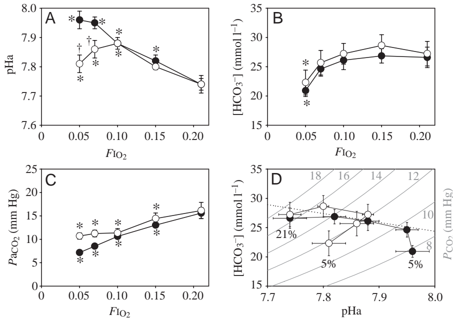
Fig. 2. Effects of hypoxia ( F_{I_{O_2}} =fraction of oxygen in the inspired air) on acid-base status before and after reducing haematocrit (filled and unfilled circles, respectively). (A) Arterial pH (pHa); (B) plasma bicarbonate concentration; (C) arterial carbon dioxide tension ( P_{aCO_2} ; 1 mm Hg=133.3 Pa) and (D) Davenport diagram. In the Davenport diagram, an in vitro buffer line previously determined by Andersen et al. (2001) is shown as a dotted line, and isobars for carbon dioxide tension have been added (grey lines). Significant effects of hypoxia within each of the two groups (normal and low haematocrit, respectively) are marked with an asterisk, and significant differences between the groups are marked with a dagger. Data are presented as means \pm 1 S.E.M. ( N=6 ).
