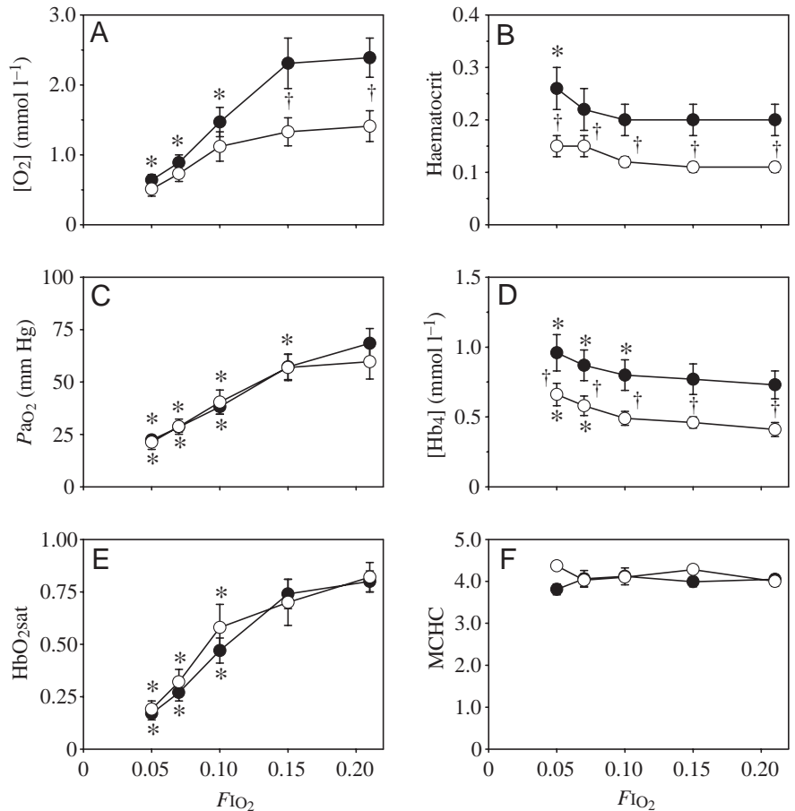
Fig. 1. Effects of hypoxia ( F_{IO_2} =fraction of oxygen in the inspired air) on arterial oxygen levels before and after reducing haematocrit (filled and unfilled circles, respectively). (A) Oxygen concentration ( [O_2] ); (B) haematocrit; (C) arterial oxygen tension ( P_{aO_2} ; 1 mm Hg=133.3 Pa); (D) haemoglobin concentration ( [Hb_4] ); (E) haemoglobin oxygen saturation ( HbO_2\text{sat} ) and (F) mean cellular haemoglobin concentration (MCHC). Significant effects of hypoxia within each of the two groups (normal and low haematocrit, respectively) are marked with an asterisk, and significant differences between the groups are marked with a dagger. Data are presented as means \pm 1 S.E.M. ( N=6 ).
